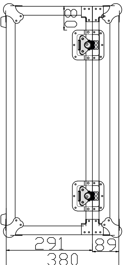
Top View 1
