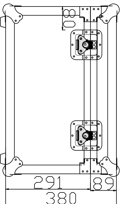
Top View
