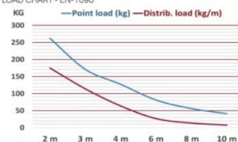
LOAD CHART - EN-1090
